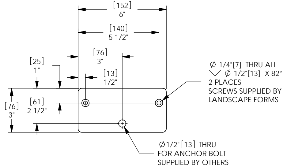
MOUNTING PLATE DETAIL
